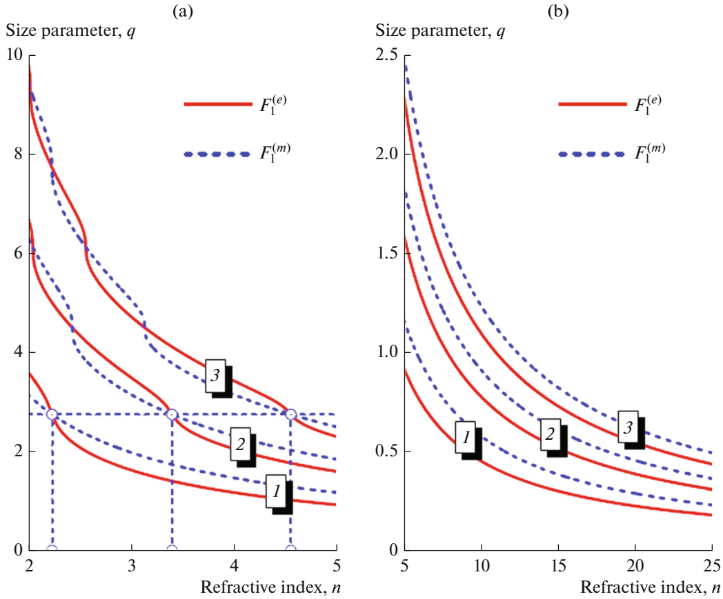
Fig. 18. (Color online) Trajectories F_1^{(e)}(n, q) = 0 (equivalent of \Re_1^{(a)} = 0 ) and F_1^{(m)}(n, q) = 0 (equivalent of \Re_1^{(b)} = 0 ), corresponding to the disappearance of electric and magnetic dipole modes in the plane of parameters n and q , for (a) n < 5 and (b) n > 5 .
