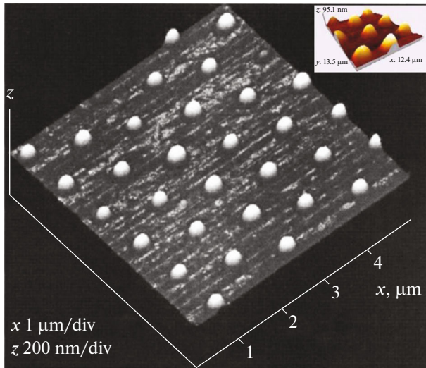
Fig. 5. (Color online) Silicon surface with nanobumps, formed as a result of silicon irradiation by a KrF laser pulse through an array of dielectric microspheres with a refractive index n = 1.6 [51].
