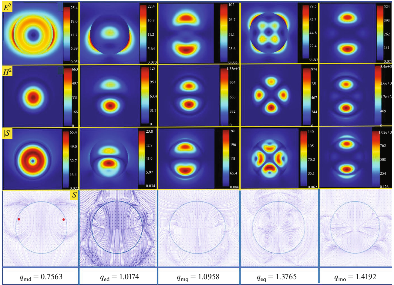
Fig. 7. Distributions of the electric intensity E^2 (first row), magnetic intensity H^2 (second row), Poynting vector modulus |S| (third row), Poynting vector lines (fourth row), and the resonant values of size parameter in the corresponding columns. The values for the first five resonances in Fig. 6 are indicated.
