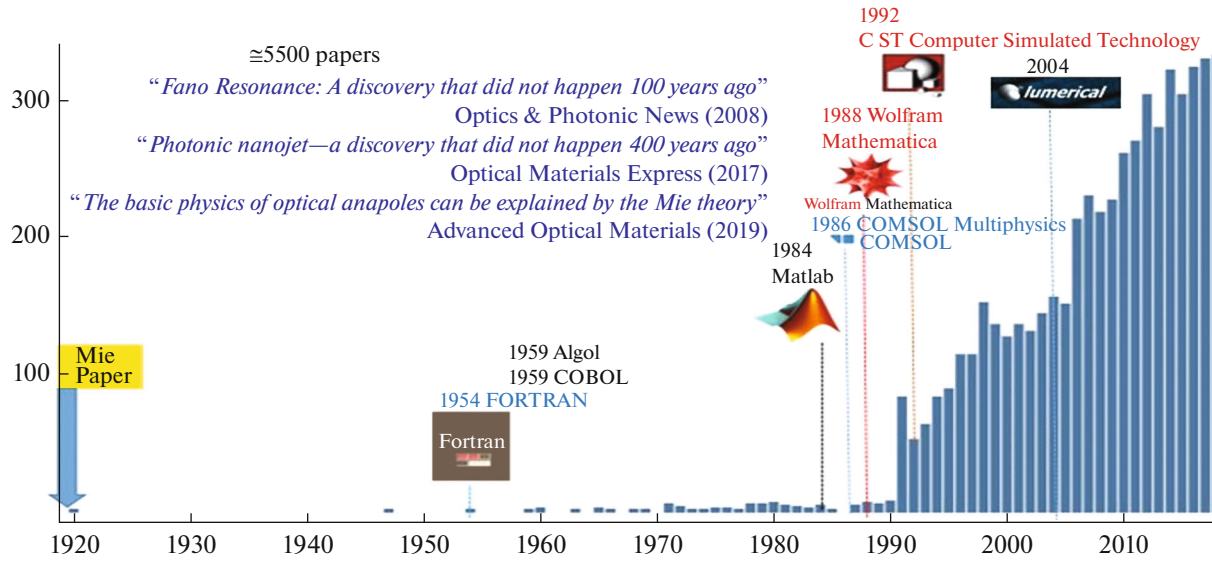
Fig. 1. (Color online) Number of publications devoted to the Mie theory, according to the Web of Science [5].
