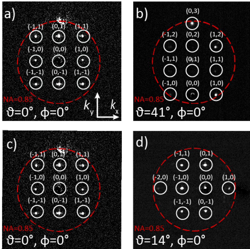
Fig. 3. (a,c) Experimental BFP images under normal incidence excitation ( \vartheta = 0^\circ ) and x-polarized light ( \phi = 0^\circ ). The red circle represents the numerical aperture of the objective (NA=0.85). (b,d) BFP images with tilted illumination at 41^\circ for p and 14^\circ for s polarized light. When the angle of incidence is increased, the (0,0) order is not emitted perpendicularly to the metasurface due to the in-plane components. For p -polarization, the diffraction orders move along k_y since the incident beam wavevector lies in the yz -plane, while, for s -polarization, they move along k_x since the incident wavevector is in the xz -plane. As a consequence, at certain angles, some diffraction orders disappear and others fall in the NA view window.
