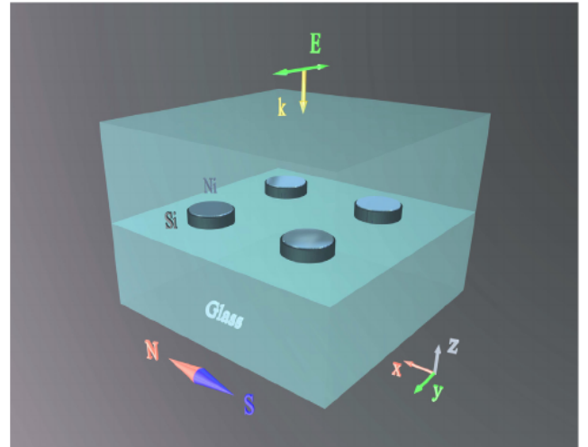
Fig. 1. Scheme of the model. 5-nm-thick nickel film covers 220-nm-thick silicon nanodisks. Subdiffractional array is organized by nanodisks with interparticle distance of 200 nm forming the magnetophotonic metasurface. The metasurface is embedded in a dielectric environment with n = 1.5 . An external magnetic field is applied along the X direction, polarization of light is oriented along Y axis and the wavevector is collinear with Z axis.
